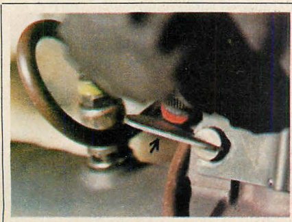
IR devices, since they have own light source, must have ability to focus IR light source with electronic telescope. On this IR unit, is accomplished via small lever mounted below IR lamp assembly.
